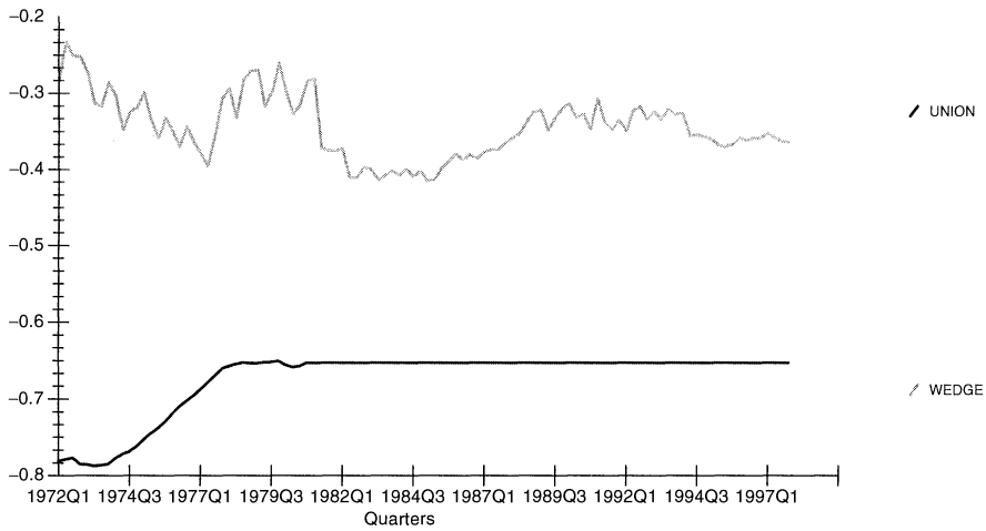
Figure 2. The wedge and the unionization variables
